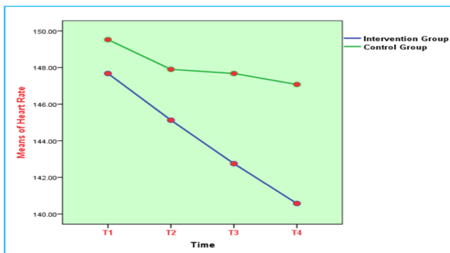
Fig.4: The Means of Heart Rate in two groups of Intervention and Control at different time periods (Repeated Measure ANOVA test).
